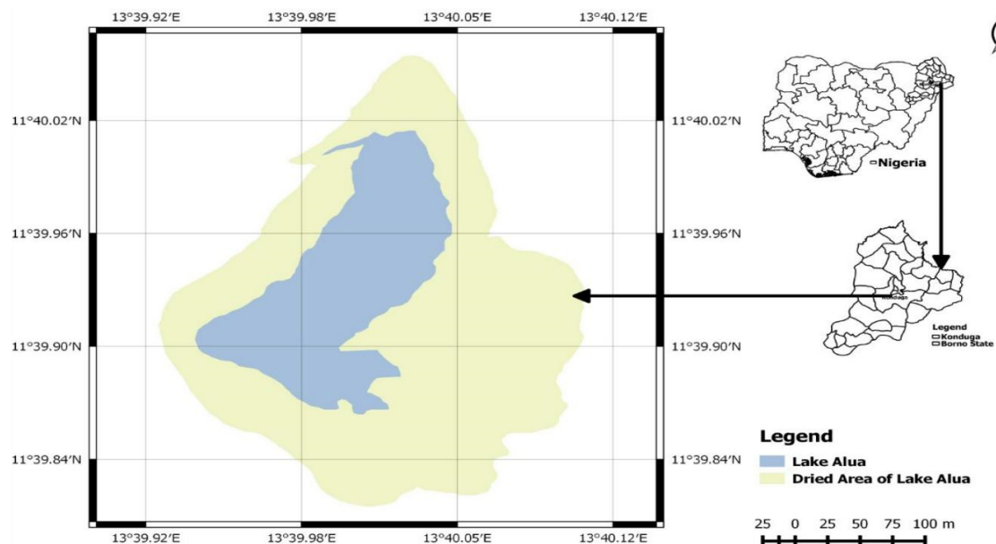
Fig. 1: Map of Lake Alau, Maiduguri, Nigeria
