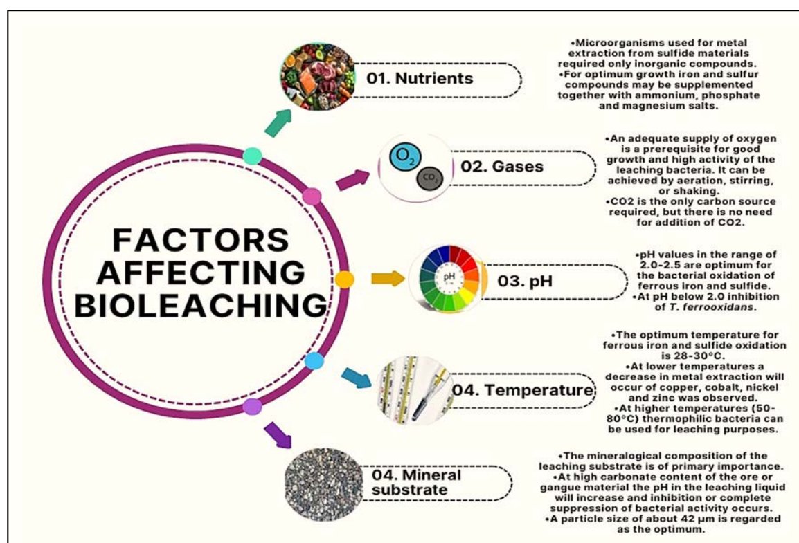
Fig. 2: Different factors that affect the process of bioleaching
