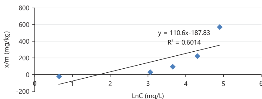
Fig. 17: Temkin's model for soils under shale mixed with sandstone and clay
