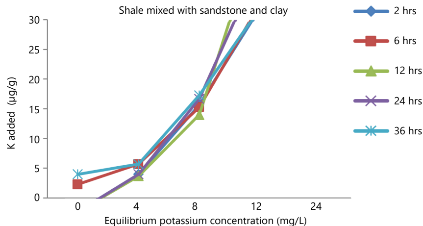
Fig. 5: Potassium adsorption characteristics of soils under shale mixed with sandstone and clay parent material as a function of time
