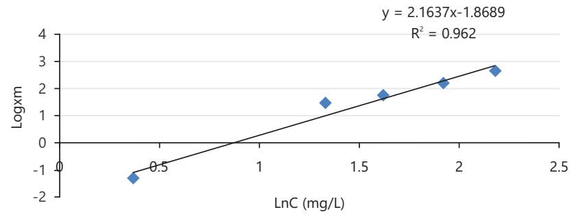
Fig. 12: Freundlich adsorption isotherm for soils under the basement complex
